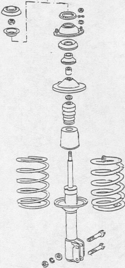
Front Strut Assy.
